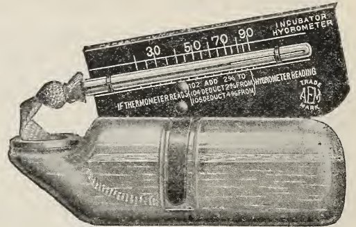
Hygrometer.
